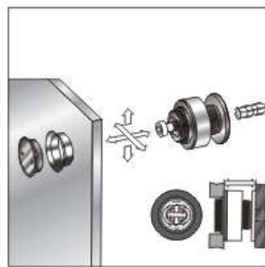
● JU800F-5 玻璃与墙体固定件 Single point fixing (可调节加强型, 调节节位18.5至24.5mm) Adjustable and strengthened, adjusted 18.5mm—24.5mm
