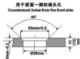
斜口连接帽 Countersunk holes connecting
