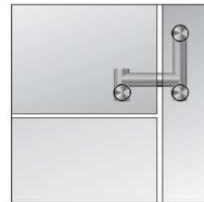
● JU800C-5 曲型固定件 Overpanel/sidelight connector
