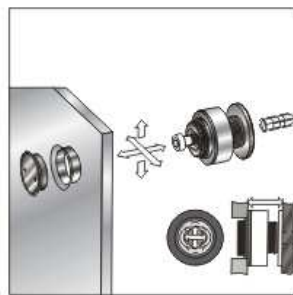
● JU800F-3 玻璃与墙体固定件 Single point fixing (可调节, 调节节位11.5至14.5mm) Adjustable, adjusted 11.5mm—14.5mm
