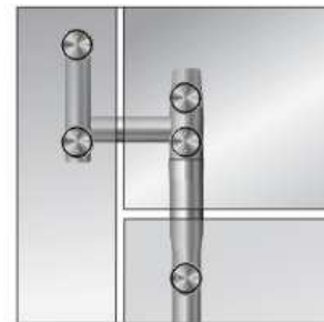
● JU800C-1 曲型顶轴 Overpanel/sidelight connector with pivot bearing location
