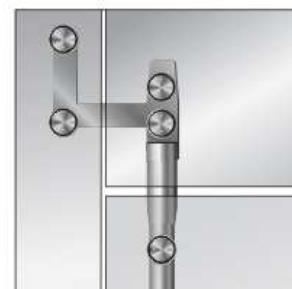
● JU800D-1 曲型顶轴 Overpanel/sidelight connector with pivot bearing location
