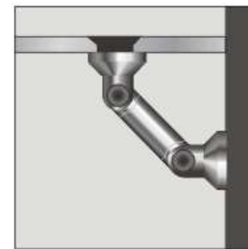
● JU800E-2 单杆固定件 Glass/wall Corner Connector (墙体与玻璃连接, 双头可调角度) Connection for connecting wall and glass, both sides can adjusted angle
