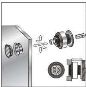
● JU800F-4 玻璃与墙体固定件 Single point fixing (可调节加强型, 调节节位14.5至18.5mm) Adjustable, adjusted 14.5mm—18.5mm
