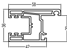
80Sliding Sash(C) T80S(C) 0.76kg/m
