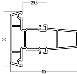
80Upper Sliding Transom T80LT 0.93kg/m
