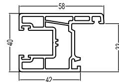
88 Sliding Sash (B) T88S (B) 0.76kg/m
