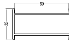
60Frame Connecting Profile 60PG 0.56kg/m
