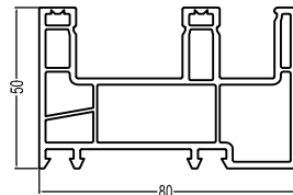
80Sliding Frame(A) T80K(A) 1.12kg/m
