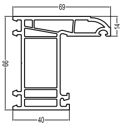
66Casement Frame (B) P66K (B) 1.19kg/m
