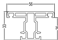
75Sash Mullion T75SZT 0.52kg/m
