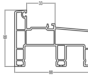
88 Transom Trame T88WLT 1.35kg/m
