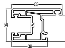
80Sliding Sash(B) T80S(B) 0.68kg/m
