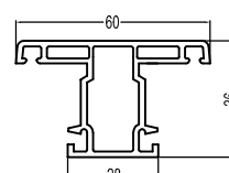
80Sash Mullion T80SZT 0.62kg/m
