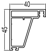
60Casement Insect Screen P60SS 0.47kg/m
