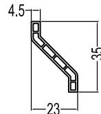
Jalousie window vane BY 0.16kg/m
