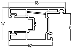
60/88Sliding Sash(A) T60/88S(A) 0.86kg/m
