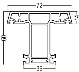
60Casement Mullion(B) P60ZT(B) 1.15kg/m
