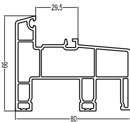
80 Transom Trame T80WLT 1.17kg/m
