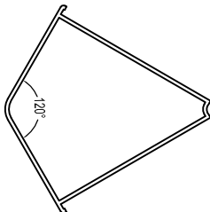
120° Corner Profile(80) 120° ZJ(80) 0.75kg/m
