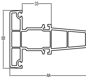
88 Upper Sliding Transom T88LT 1.07kg/m
