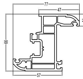
66Inswing Sash(C) P66NKCS (C) 1.17kg/m
