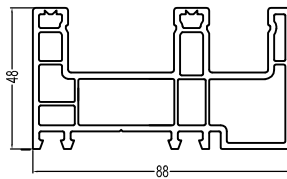
88 Sliding Frame (B) T88K (B) 1.25kg/m
