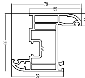
66Inswing Sash(A) P66NKCS (A) 1.23kg/m
