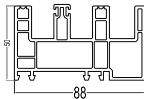
88 Four Track Sliding Frame T88SGK 1.35kg/m
