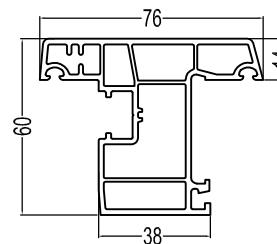
60 Outswing Sash P60WKCS 1.05kg/m
