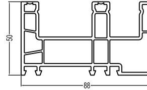
88 Sliding Frame (C) T88K (C) 1.34kg/m
