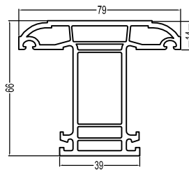
66Casement Mullion(A) P66ZT (A) 1.21kg/m
