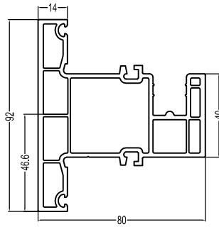
80 Sliding Tranlatory Mullion(A) PT80ZT (A) 1.6kg/m
