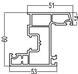
60Inswing Sash(A) P60NKCS(A) 1.05kg/m
