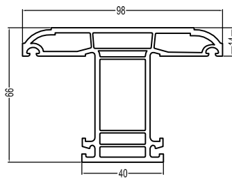
66Casement Mullion(B) P66ZT (B) 1.35kg/m
