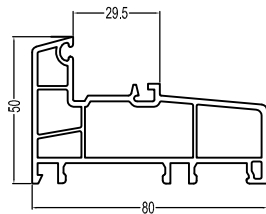
80Upper Sliding Frame T80LK 0.9kg/m
