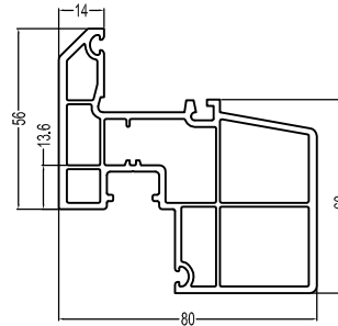
80 Sliding Tranlatory Big Sash(A) PT80DS (A) 1.39kg/m
