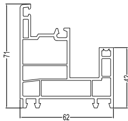
75 Single Sliding Frame T75DK 1.0kg/m
