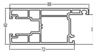
60Sliding Sash(B) T60S(B) 1.1kg/m
