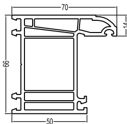
66Casement Frame (A) P66K (A) 1.23kg/m
