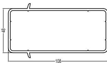
Big Frame Connecting Profile DPG 1.05kg/m
