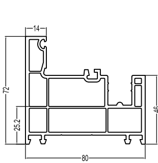
80 Sliding Tranlatory Frame(A) PT80K (A) 1.45kg/m
