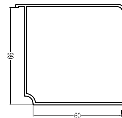
60/66Corner Profile(90) 60/66FZJ(90) 0.75kg/m
