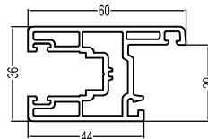
80Sliding Sash(A) T80S(A) 0.76kg/m
