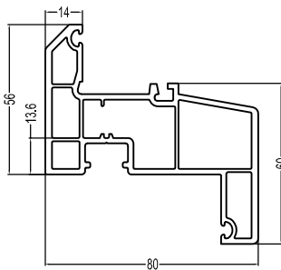
80 Sliding Tranlatory Small Sash(A) PT80XS (A) 1.29kg/m
