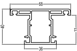
60/88Sash Mullion T60/88SZT 0.7kg/m
