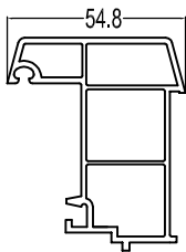
60Inswing Mullion P60NKFT 0.7kg/m
