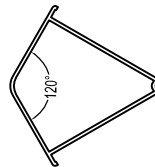
120° Corner Profile(60/66) 120° ZJ(60/66) 0.57kg/m
