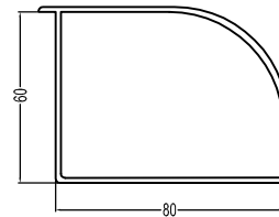
80/60Corner Profile(90) 80/60ZJ(90) 0.77kg/m
