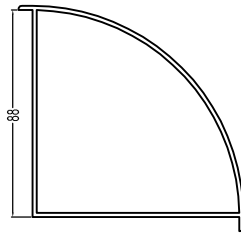
88Corner Profile(90) 88ZJ(90) 0.97kg/m
