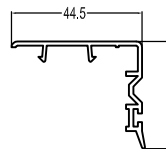
60/88Weather Strip(A) T60/88FG(A) 0.24kg/m
