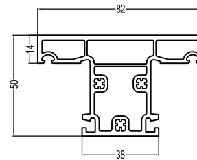
80 Sliding Tranlatory Sash Mullion(A) PT80SZT (A) 1.2kg/m
