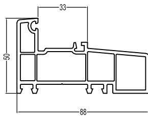
88 Upper Sliding Frame T88LK 1.06kg/m
