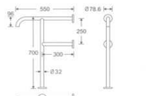
002.SS.102 Material:Stainless Stell Finish:Polished (PSS) 材质:不锈钢 表面处理:磨砂
