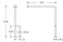
002.SS.115 Material:Stainless Stell Finish:Polished (PSS) 材质:不锈钢 表面处理:磨砂
