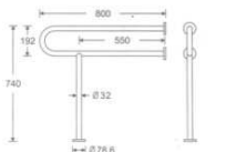
002.SS.103 Material:Stainless Stell Finish:Polished (PSS) 材质:不锈钢 表面处理:磨砂
