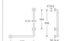
002.SS.101 Material:Stainless Stell Finish:Polished (PSS) 材质:不锈钢 表面处理:磨砂
