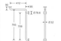
002.SS.107 Material:Stainless Stell Finish:Polished (PSS) 材质:不锈钢 表面处理:磨砂
