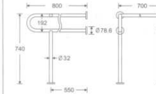
002.SS.112 Material:Stainless Stell Finish:Polished (PSS) 材质:不锈钢 表面处理:磨砂
